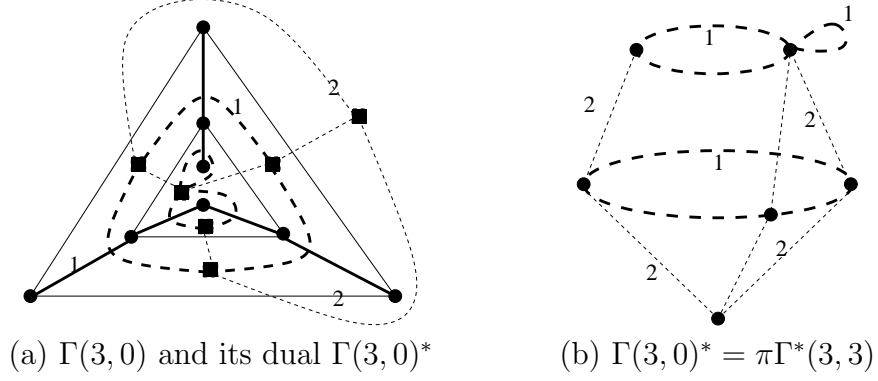
Figure 7: An Example of Capped Cylinder Graph and its Dual for \Gamma = \{\{0, 1\}, \{2\}\}
