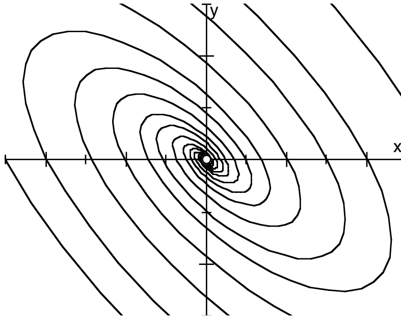
Phase plane of (2).
