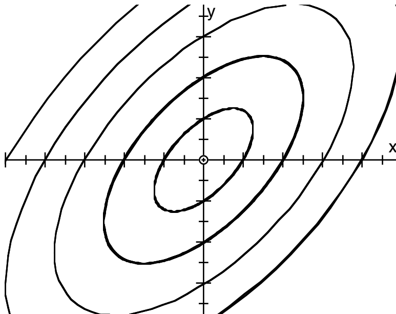
Phase plane of (1).
