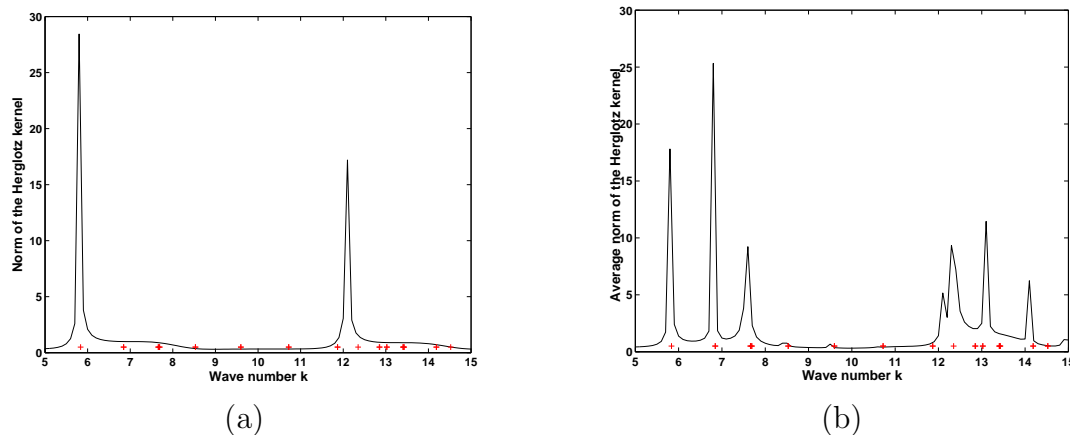
Figure 1. Results for the circle using the isotropic coefficient in (38). a) the norm of the Herglotz kernel using the single auxiliary source point z = (0, 0) . Crosses show the real transmission eigenvalues predicted by the finite element code. Only the eigenmodes associated with J_0 are visible from the kernel calculation. b) the average norm of the Herglotz kernel using 25 randomly chosen points inside the circle. Now other eigenvalues are detected.
