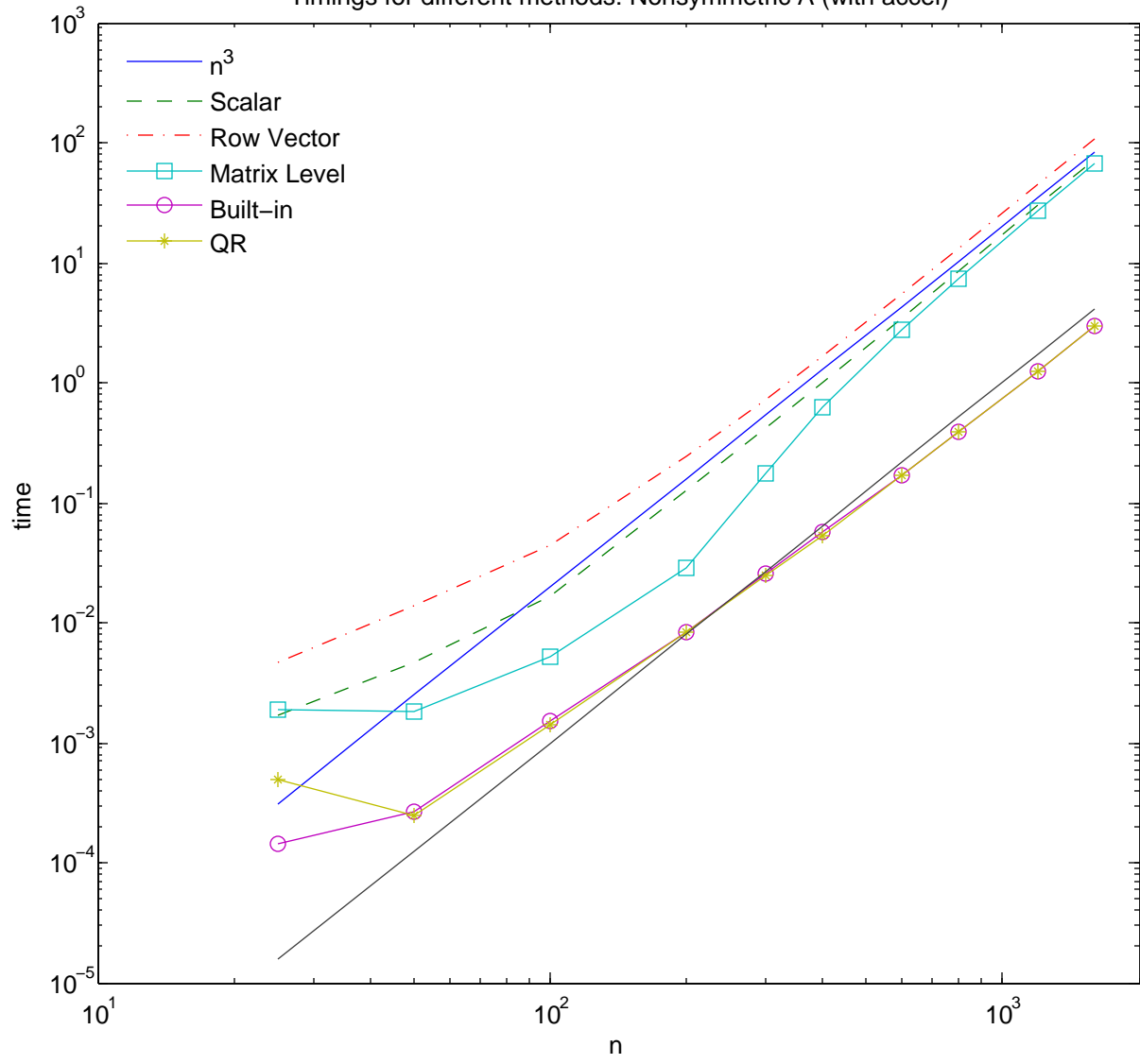
Timings for different methods: Nonsymmetric A (with accel)
