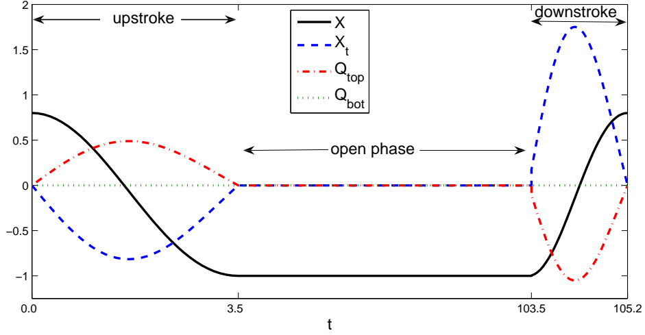
Figure 3: An example of the lid motion X(t) , lid speed X_t(t) , boundary fluxes Q_{bot} = 0 and Q_{top} = -X_t h_e with \lambda = 0.1 for FPLM boundary conditions. Note that the t axis is not to scale.
