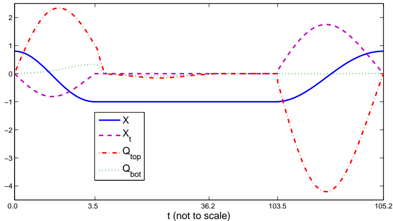
Figure 4: An example of the lid motion X(t) , lid speed X_t(t) and boundary fluxes Q_{bot} and Q_{top} with \lambda = 0.1 for FPLM+ boundary conditions. The lacrimal gland supply is approximated with Q_{olg} given by (2.20), matching the 1.2\mu\text{l}/\text{min} average flux and the punctal drainage flux given by (2.21) to conserve the tear volume over the blink cycle.
